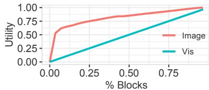
Figure 3: Utility function for image exploration application using structural similarity (red) and the visualization application which uses the system default linear function (blue).
