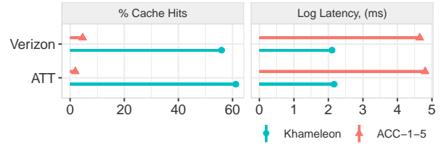
Figure 13: Performance on time-varying cellular networks.
