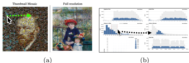
Figure 1: Two DVE applications. (a) Image exploration: hover over the left thumbnails mosaic to load full image on the right. (b) Falcon visualization [51]: drag and resize range filters in a subset of charts to update the others. We use these in our experiments §6.
