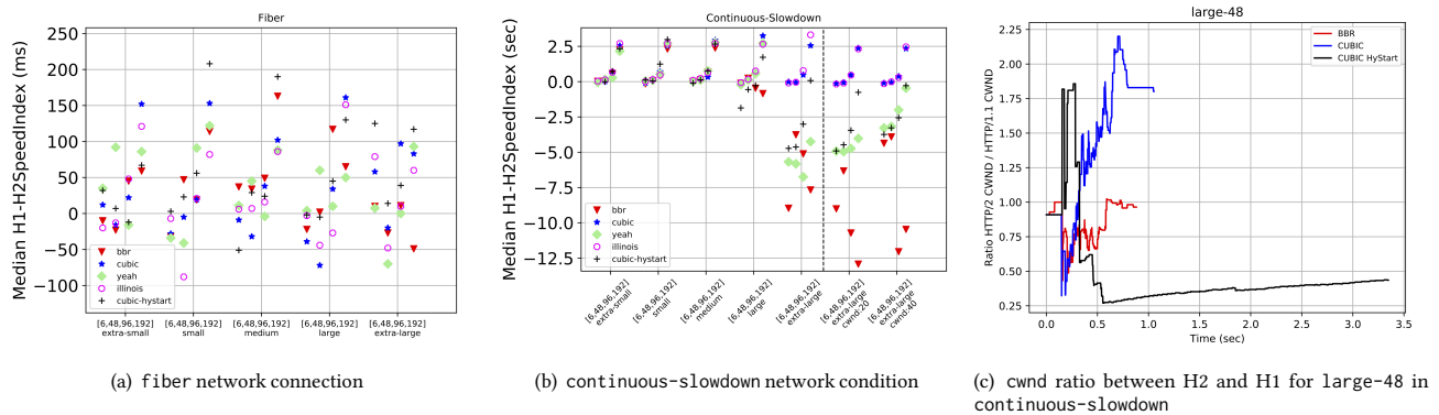
Figure 1: Difference in median SpeedIndex across 10 runs. Values > 0 indicate H2 was faster than H1, and vice-versa.
