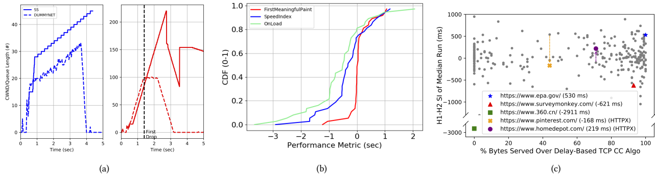
Figure 2: (a) Ground truth cwnd (SS, solid) vs Dummynet queue sampling (Dummynet, dashed). HyStart (Left) vs Slow-start (Right). MTU=500B, Object=160KB; (b) CDF of FMP/SI/PLT for (large, 48, cubic-hystart) measured from 12 different physical locations on mobile; (c) Bytes Served Over Delay-Based TCP CC Algo for Tranco Top 300 Websites
