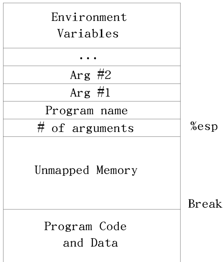
Memory Layout of a Linux Program at Startup
