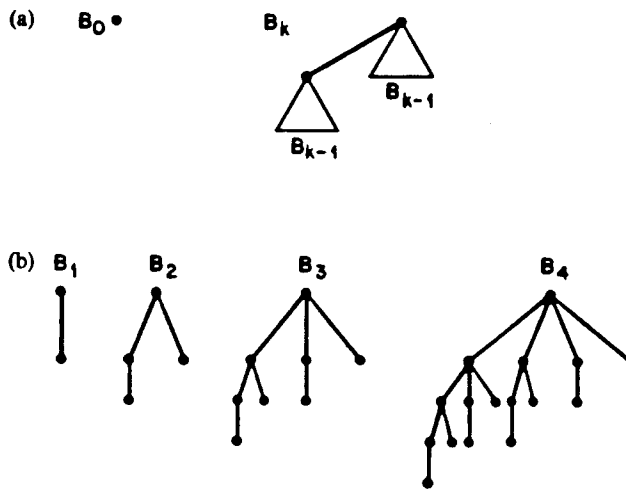
FIG. 4. Binomial trees. (a) Inductive definition. (b) Examples.
